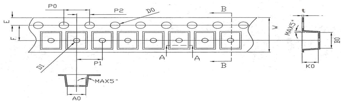
(1) Tape Dimensions(Unit:mm)
