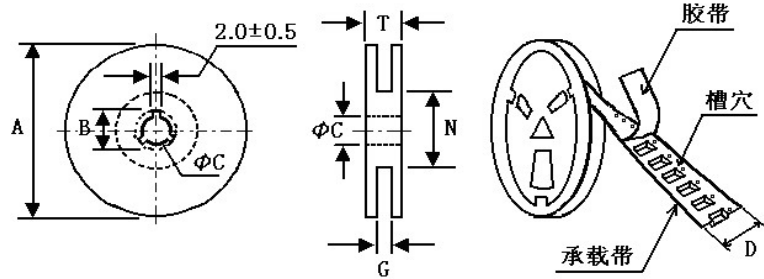
(2) Reel Dimensions (Unit:mm)
